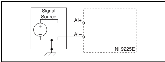
Figure 3. Connecting a Grounded Signal Source to the NI 9225E
