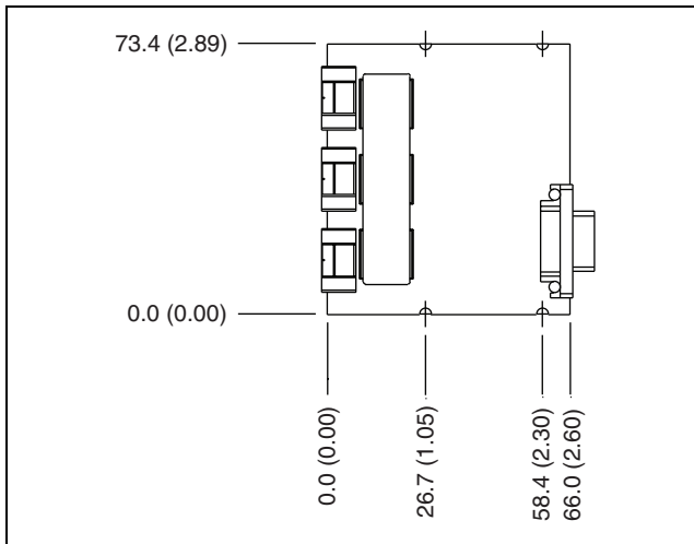
Figure 1. NI 9225E Dimensions in Millimeters (Inches)
