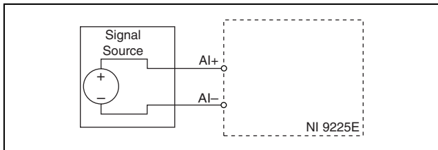
Figure 4. Connecting a Floating Signal Source to the NI 9225E
