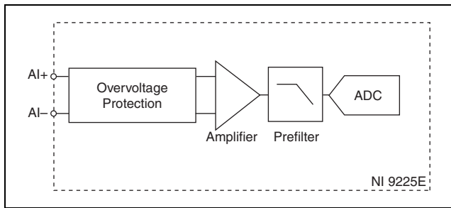
Figure 5. Input Circuitry for One Channel of the NI 9225E
