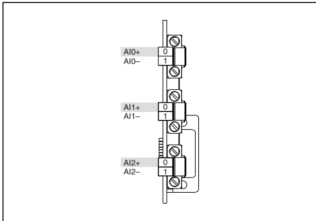
Figure 2. NI 9225E Terminal Assignments
