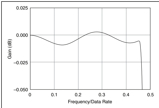
Figure 6. Typical Passband Response of the NI 9225E
